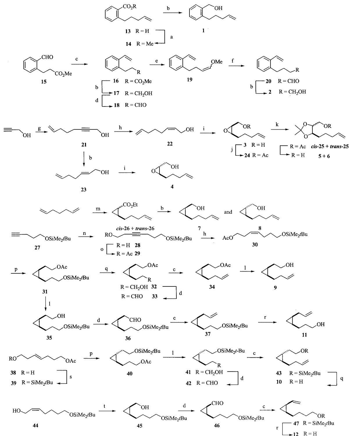
Scheme 2. a: MeOH/H + (75%); b: LiAlH 4 , THF (1: 93%; 17: 80%; 2: 98%; 23: 80%; 7: 96%; 8: 83%); c: [Ph 3 P + CH 3 ]Br - , n BuLi, THF (16: 40%; 34: 53%; 37: 93%; 43: 81%; 47: 87%); d: (COCl) 2 , DMSO, NEt 3 , CH 2 Cl 2 (18: 90%; 33: 83%; 42: 73%; 46: 87%); e: [Ph 3 P + CH 2 OMe]Cl - , n BuLi, THF (46%); f: HClO 4 , THF (80%); g: 1-bromo-4-pentene, NH 3 , LiNH 2 (97%); h: H 2 (1 atm), Lindlar catalyst (22 in acetone: 90%; 30 in hexane: 95%); i: VO(acac) 3 , t BuOOH, benzene (3: 72%; 4: 75%); j: vinyl acetate, t BuOMe, PS lipase (95%); k: BF 3 ·Et 2 O, acetone (95%); l: K 2 CO 3 , MeOH (5, 6: 95%; 9: 70%; 35: 95%; 41: 99%); m: N 2 CHCO 2 Et, Rh 2 (OAc) 4 , benzene (60%); n: ethylene oxide, n BuLi, THF (82%); o: Ac 2 O, DMAP, THF (77%); p: Et 2 Zn, CH 2 Cl 2 , (CH 2 Cl) 2 (31: 90%; 40: 93%); q: n Bu 4 N + F - , THF (32: 100%; 10: 82%); r: MeOH, cat. ClSiMe 3 (11: 86%; 12: 93%); s: imidazole, THF, ClSiMe 2 tBu (94%); t: Et 2 Zn, CH 2 I 2 , toluene, -40 °C (92%)
